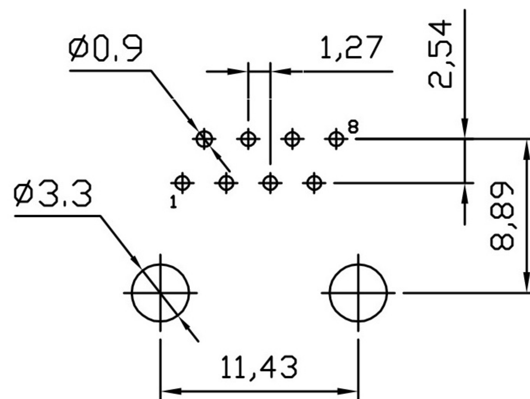
PC Board Layout Component Side Shown
