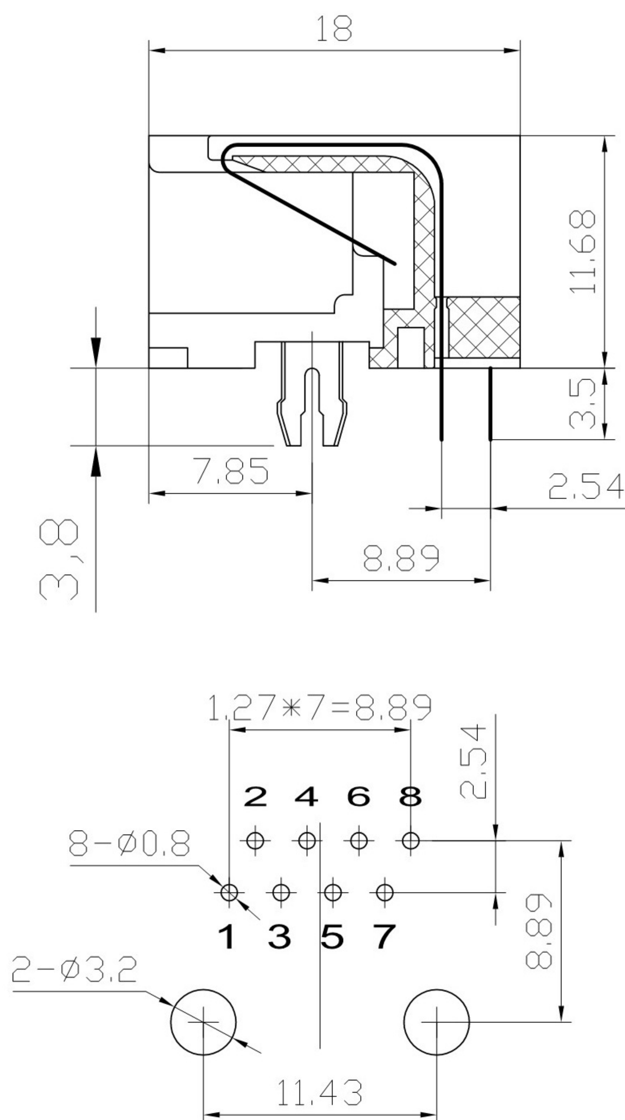
PC Board Layout Component Side Shown
