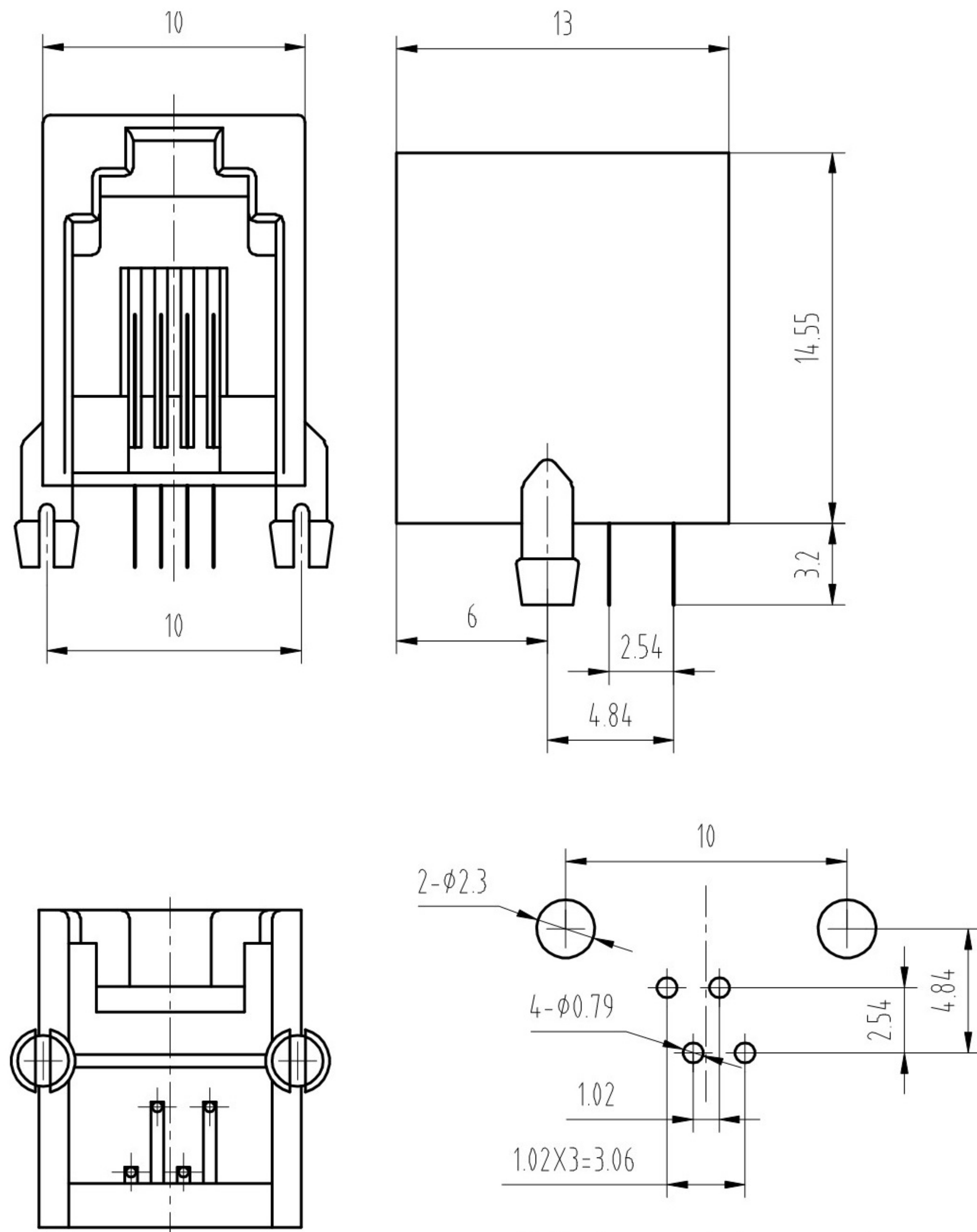
PC Board Layout Component Side Shown
