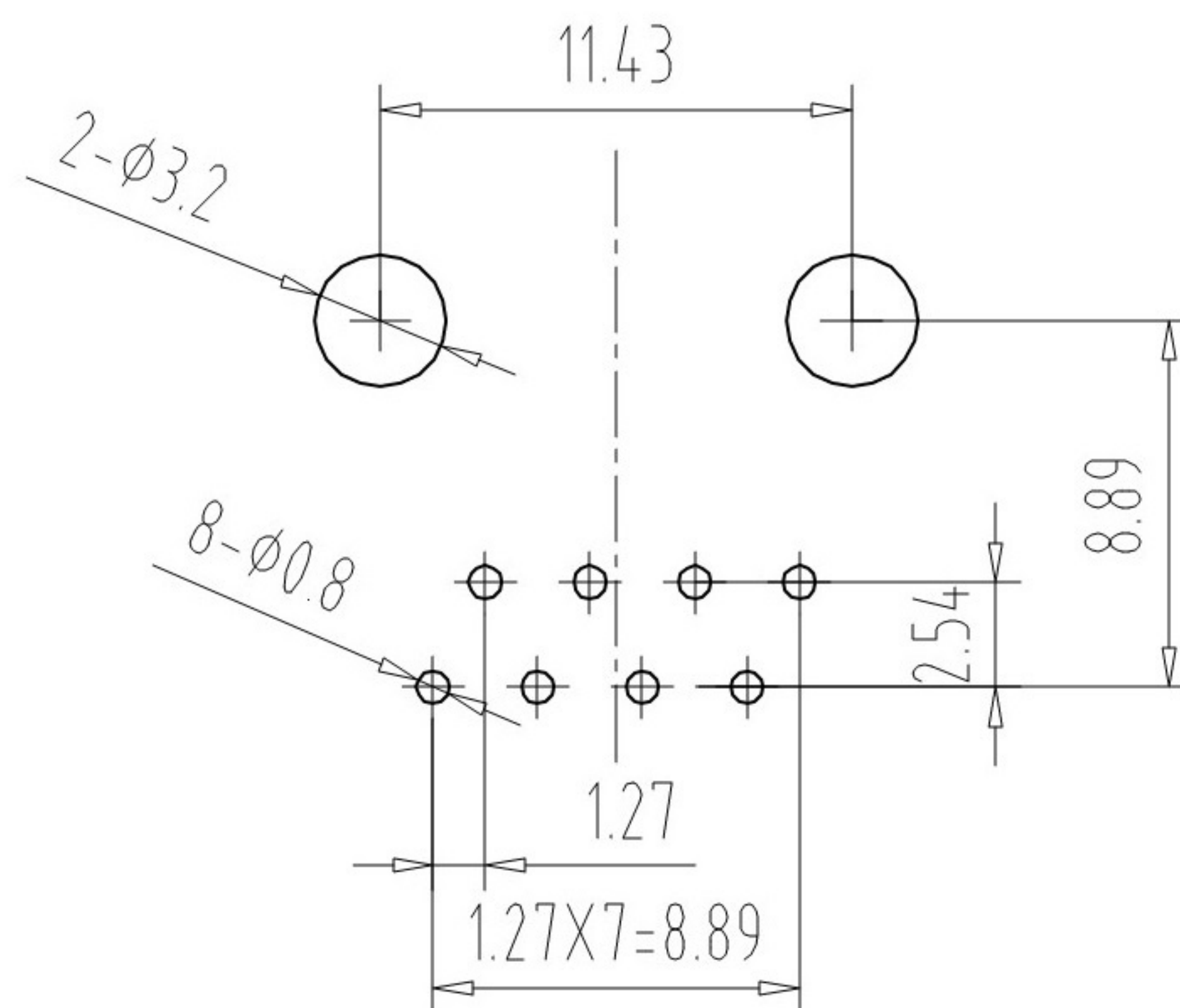
PC Board Layout Component Side Shown
