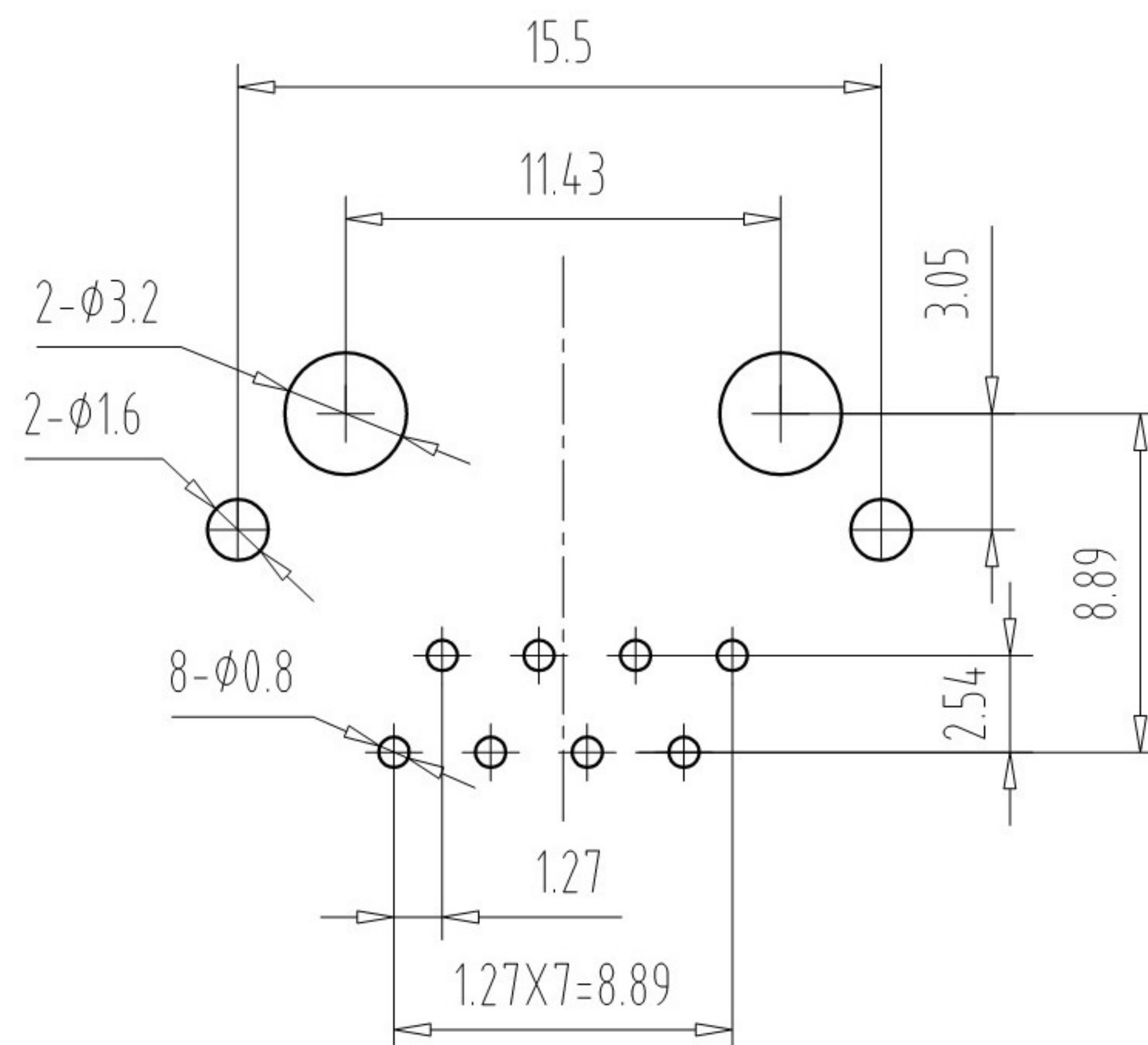
PC Board Layout Component Side Shown
