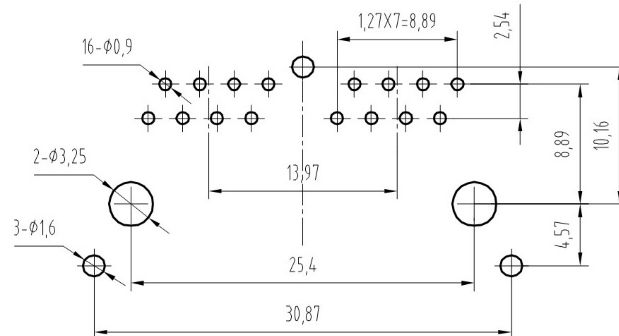
PC Board Layout Component Side Shown
