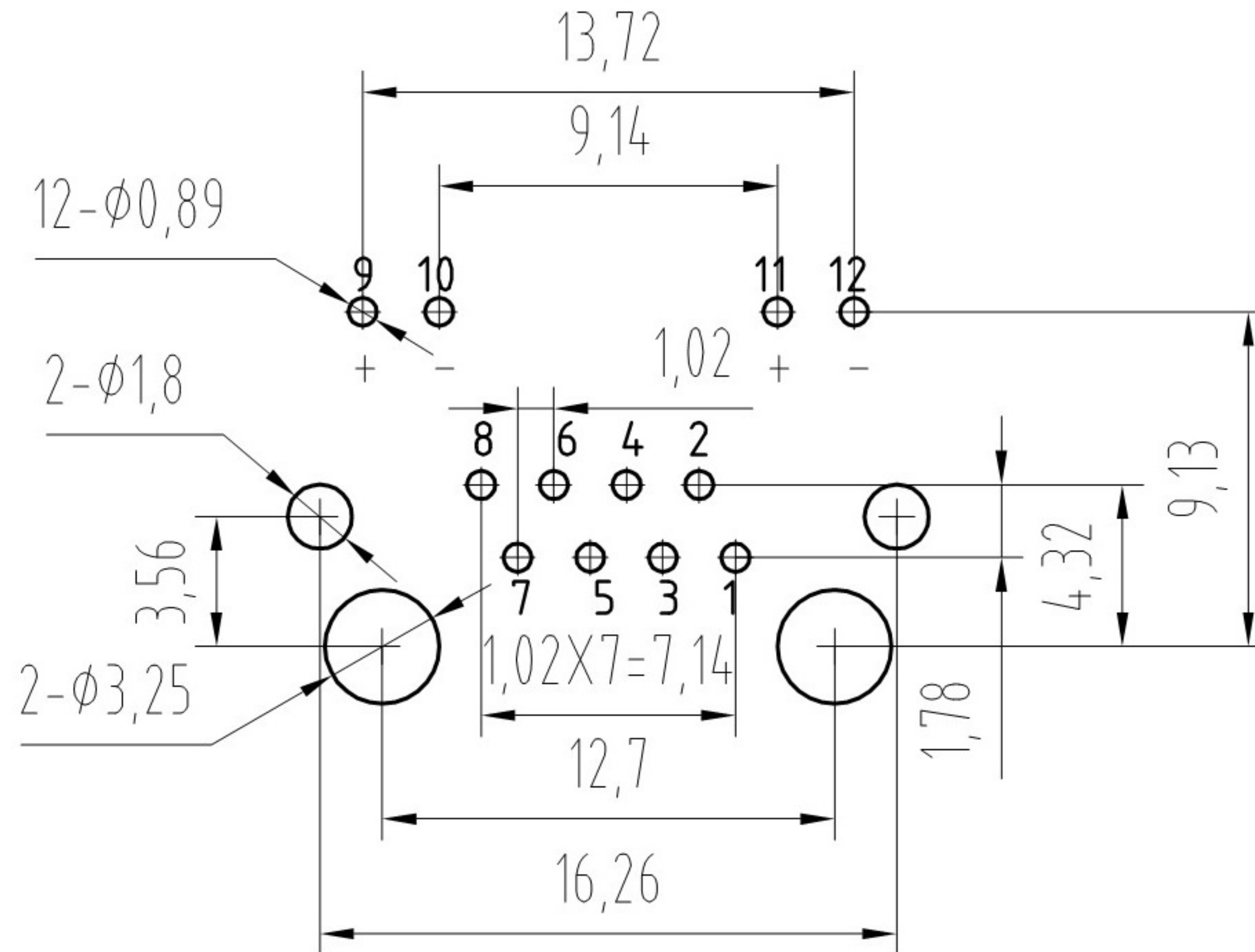
PC Board Layout
