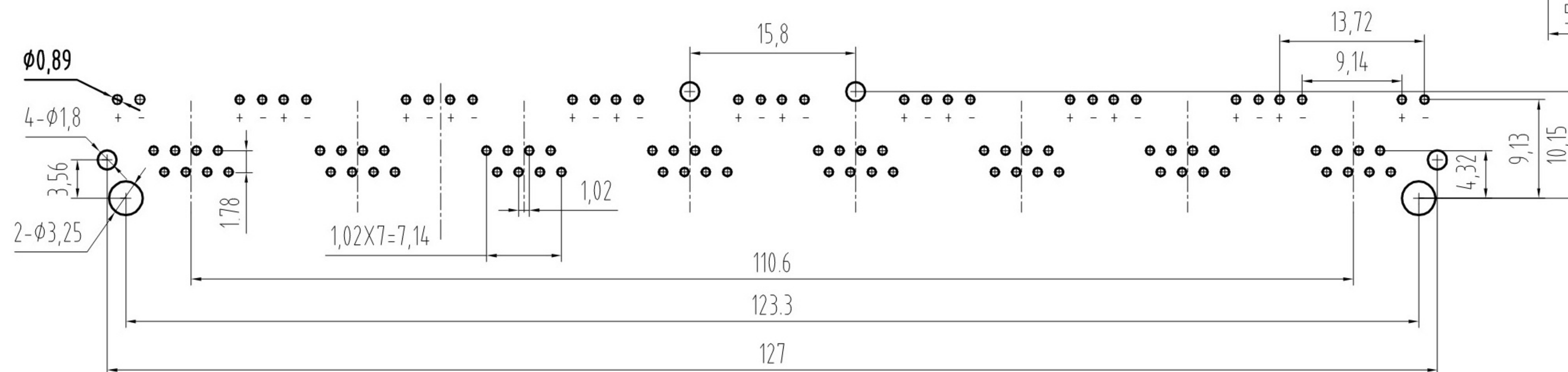
PC Board Layout Component Side Shown
