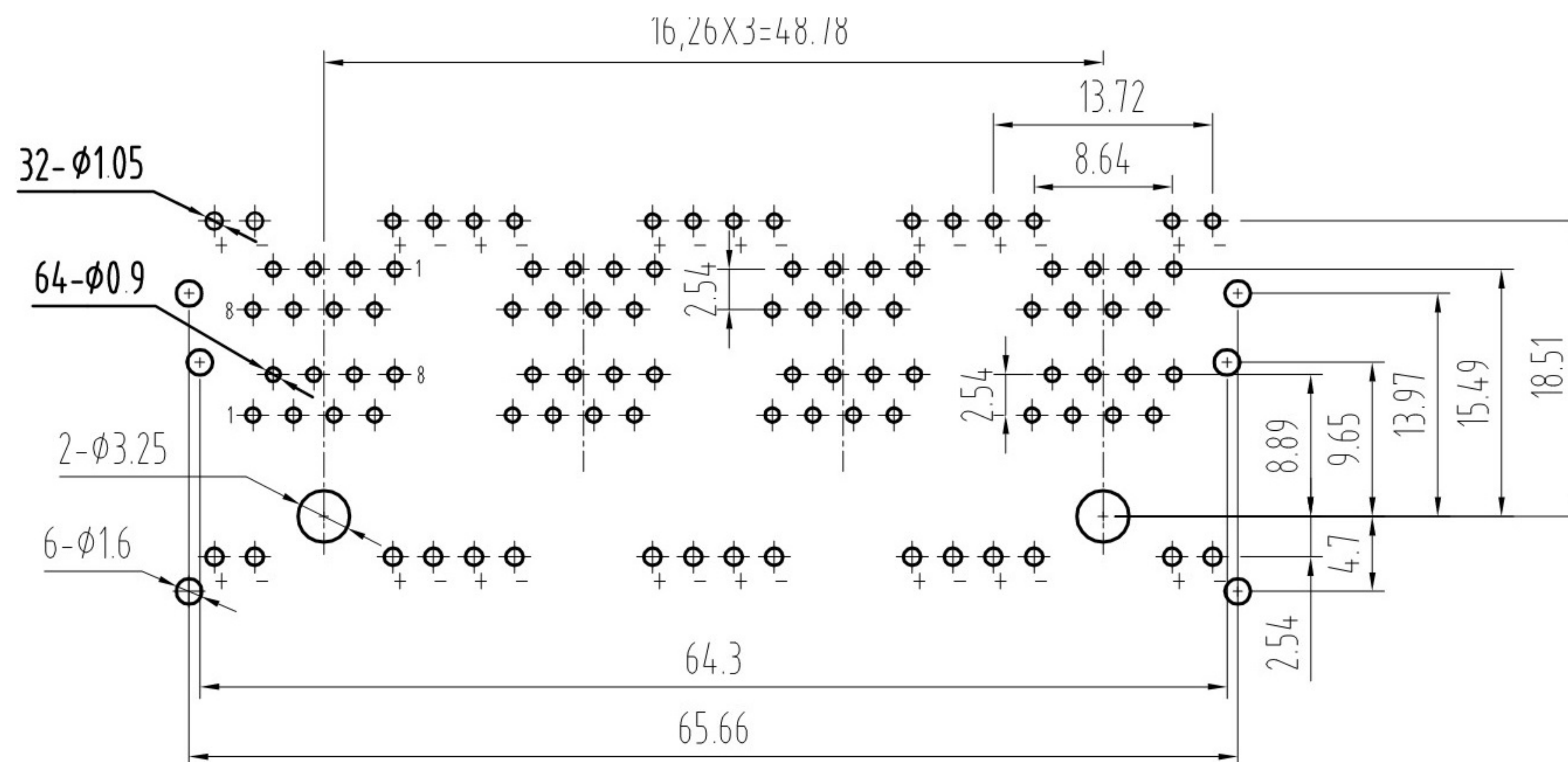
PC Board Layout Component Side Shown
