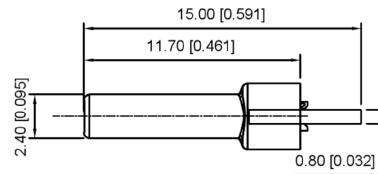
SECT B-B
