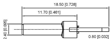
SECT B-B
