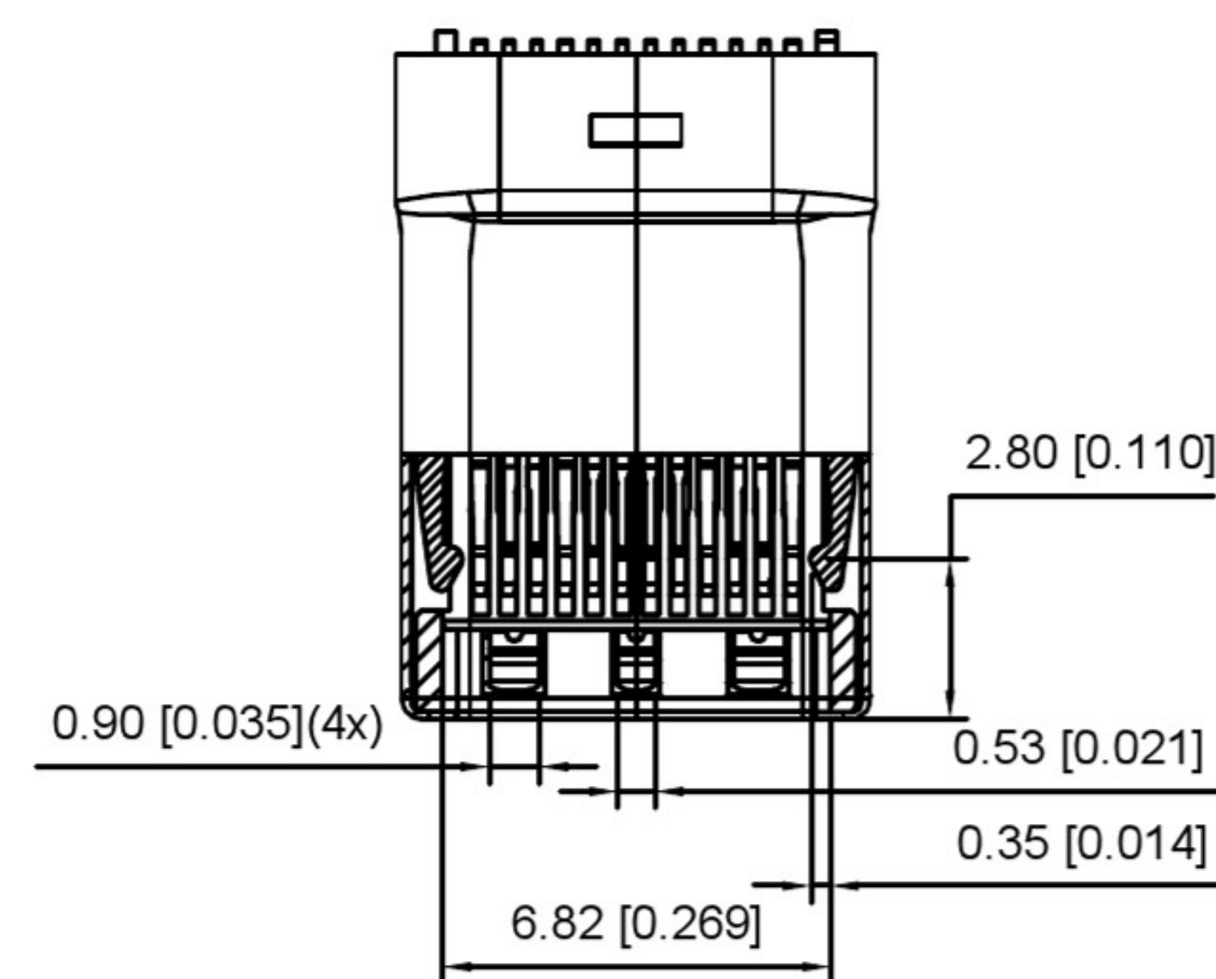
SECT B-B
