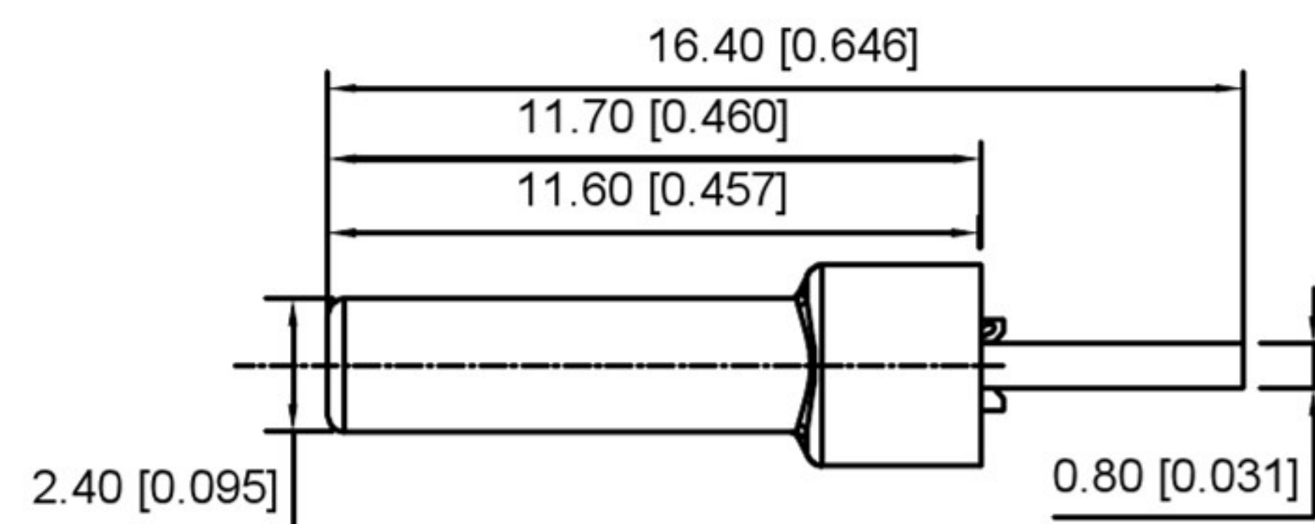
SECT B-B
