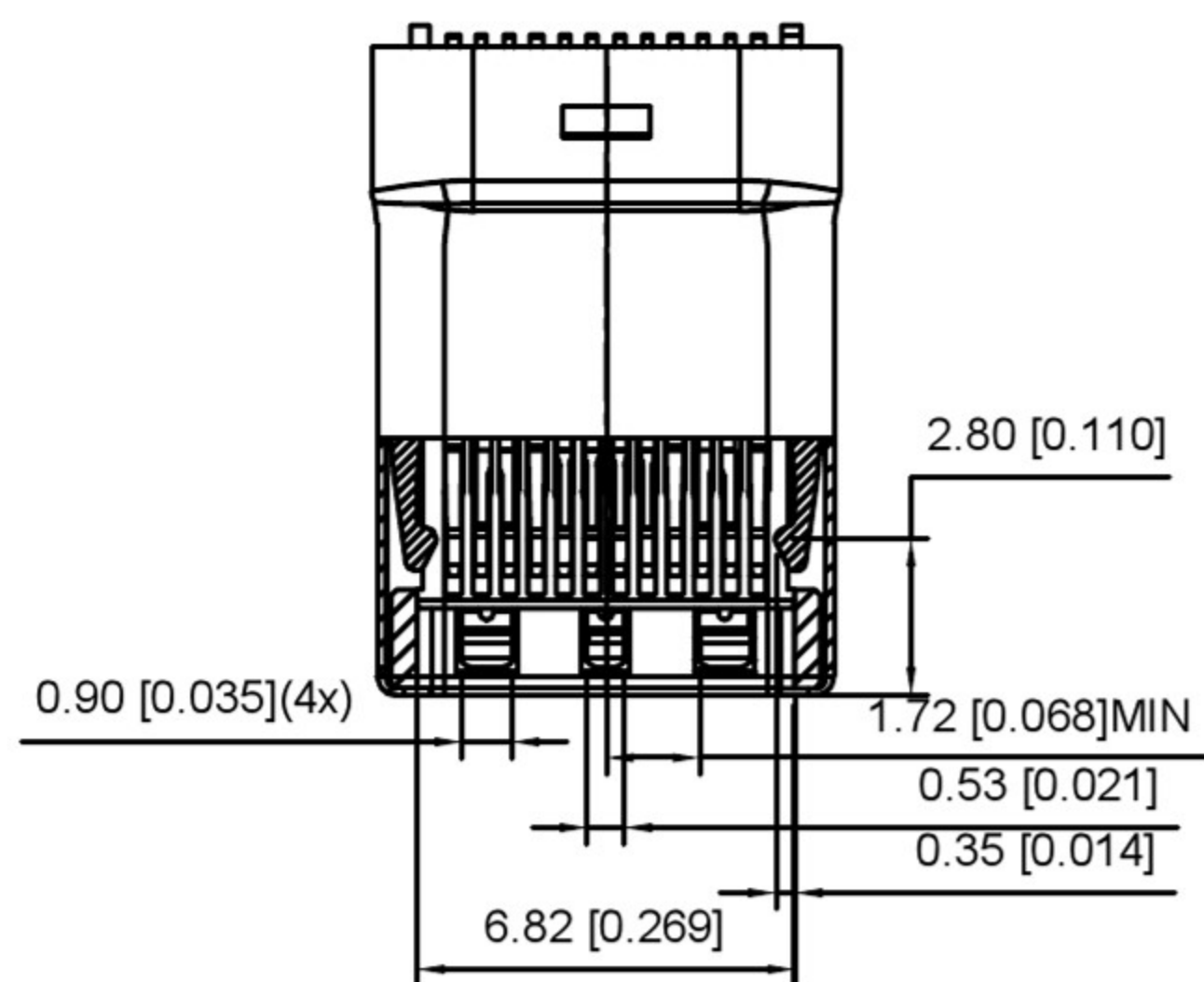
SECT B-B
