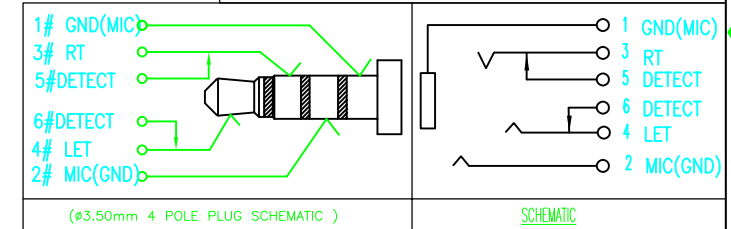
(ø3.50mm 4 POLE PLUG DETAIL DRAWING)
