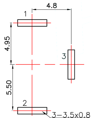
P.C.B LAYOUT(Copper-side view)
