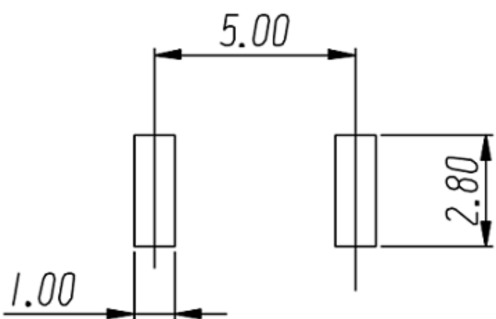
PCB LAYOUT TOP VIEW (TOLERANCE: \pm 0.05 )
