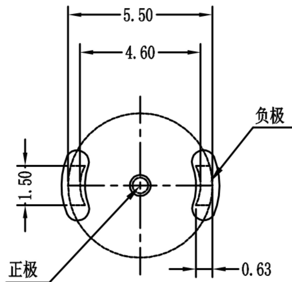
PCB LAYOUT TOP VIEW
