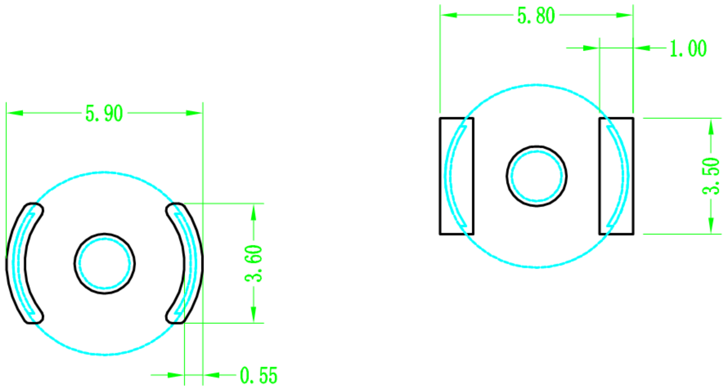
PCB LAYOUT TOP VIEW
