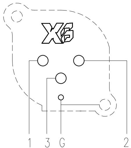
Electrical schematic
