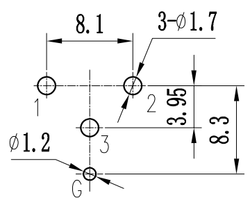
P.C.B LAYOUT (TOP VIEW) Tolerance: ±0.05
