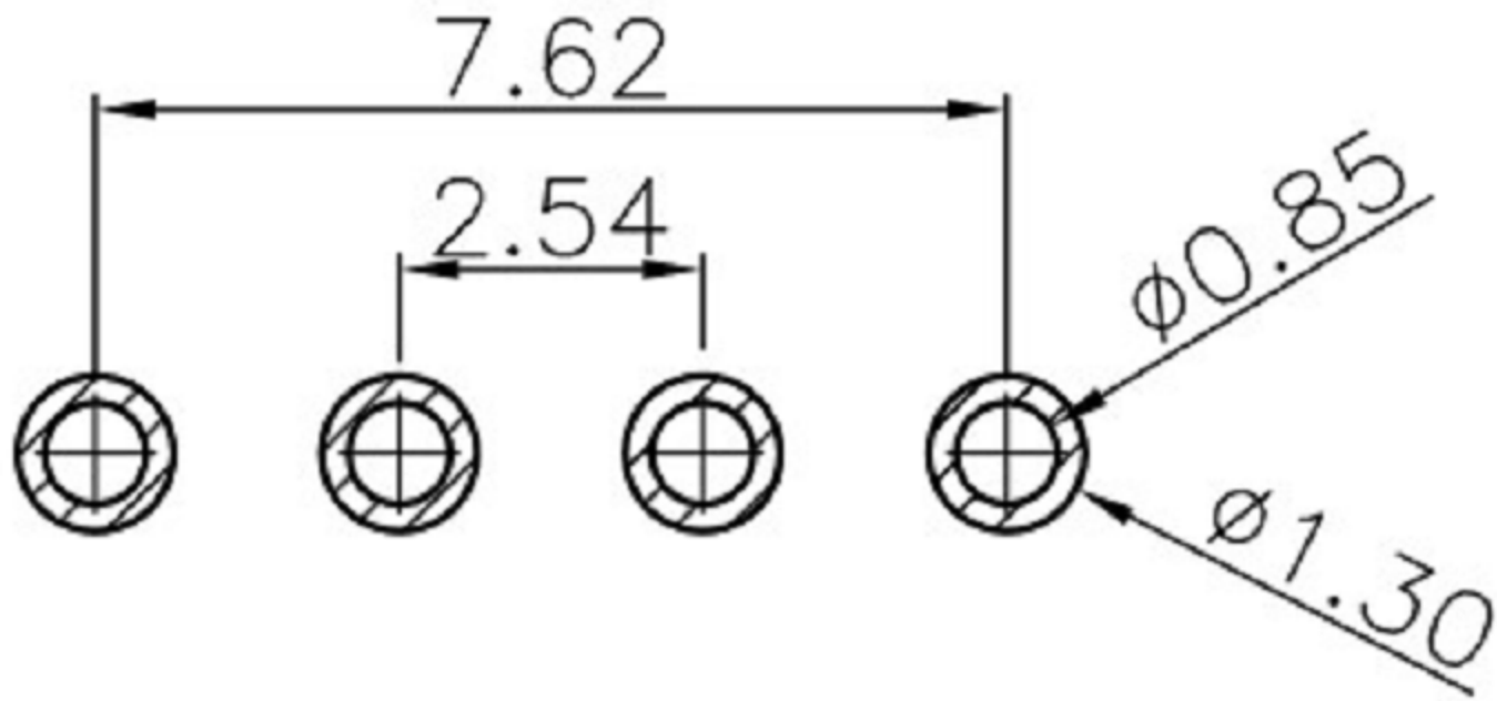
Recommended layout General tolerance: ±0.05mm
