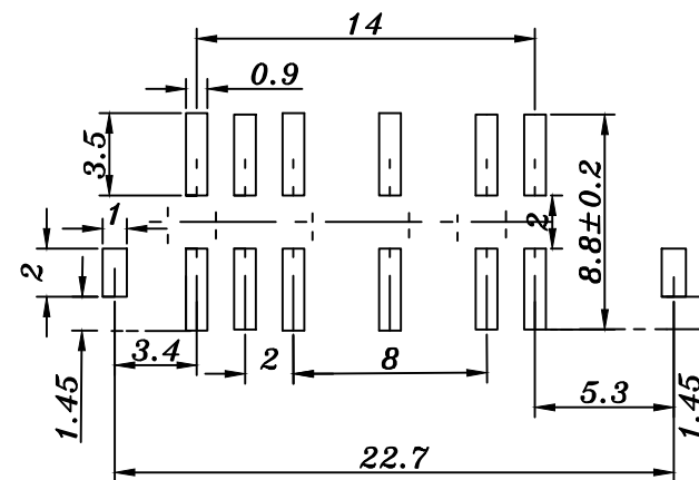
PCB LAYOUT
