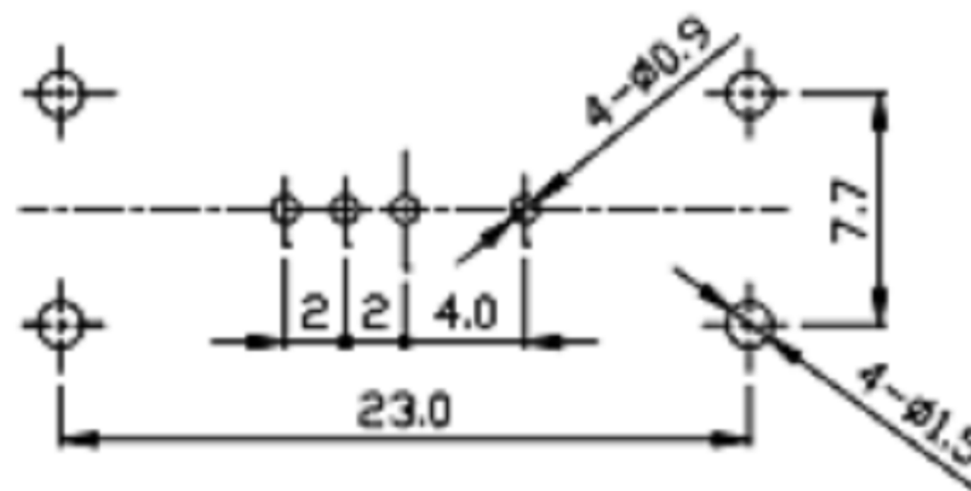
PIERCING PLAN
