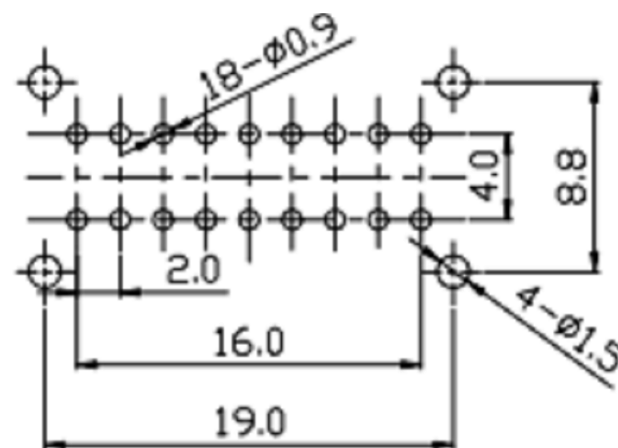
PIERCING PLAN
