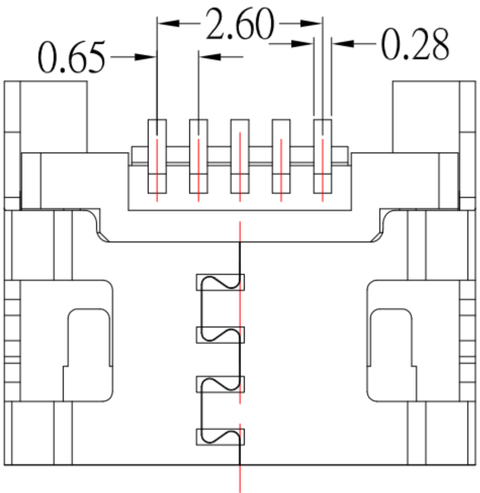
P.C.B LAYOUT MOUNTING PATTERN
