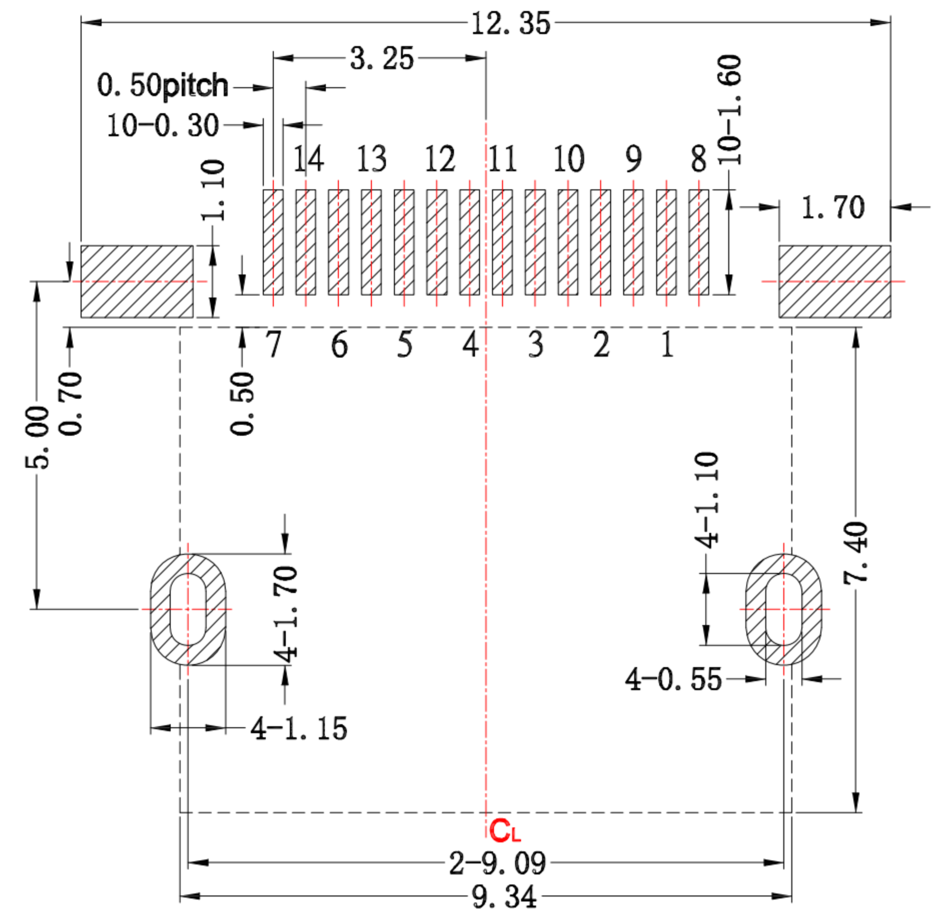
P.C.B LAYOUT MOUNTING PATTERN
