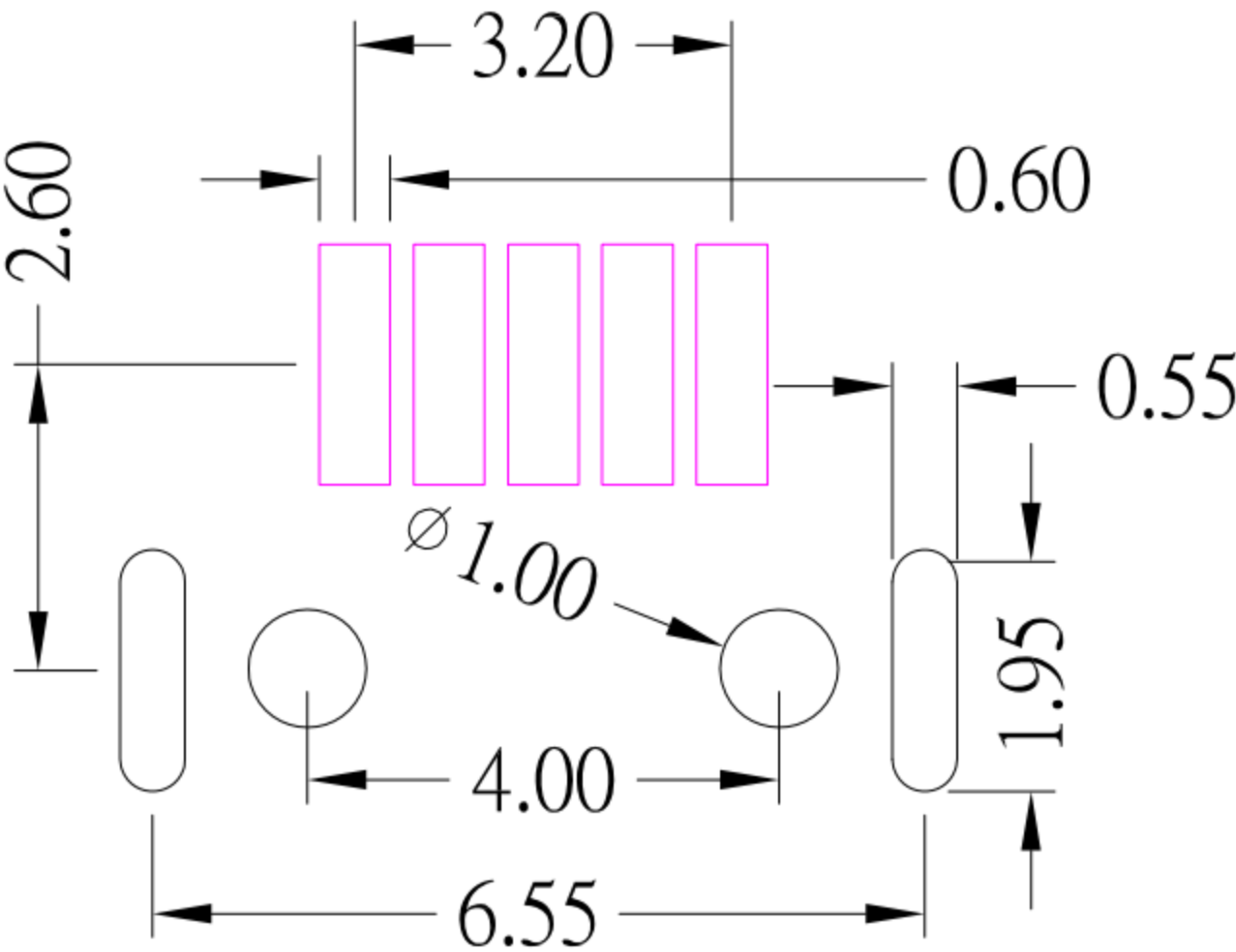
RECOMMANDED P.C.B LAYOUT
