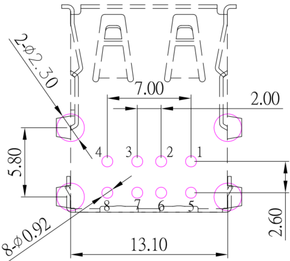
PCB LAYOUT
