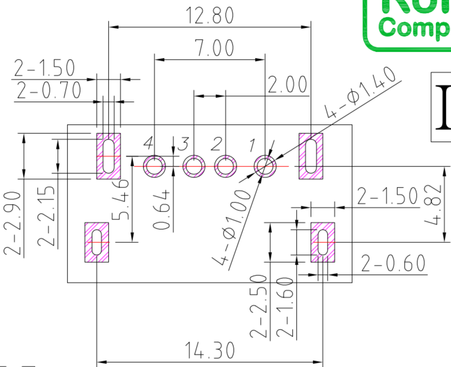
PCB LAYOUT
