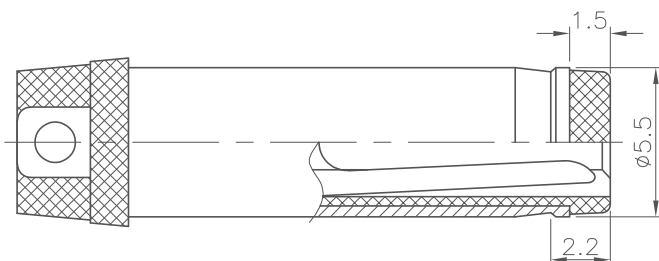
RECOMMENDED PLUG
