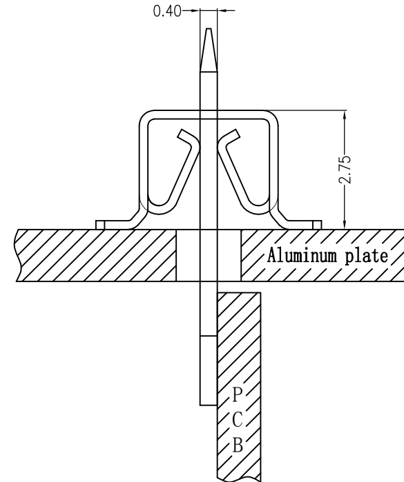
Assembly Layout
