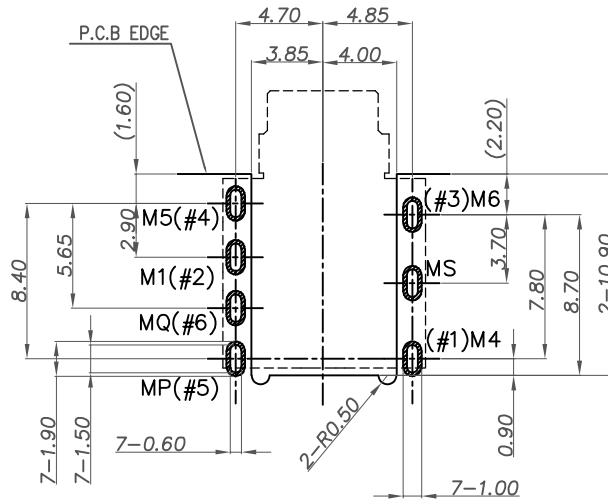
RECOMMENDED PADS LAYOUT <TOP VIEW>
