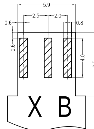
Mating Aluminum plate detail
