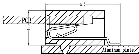
Assembly Layout
