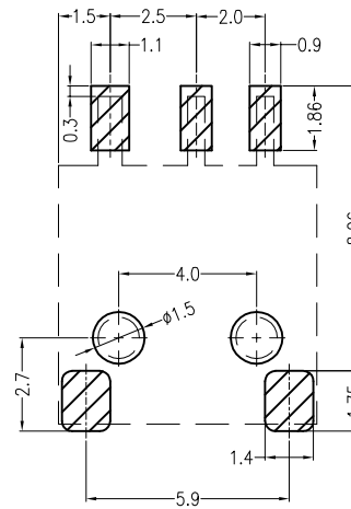
Board Layout
