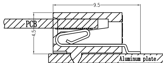
Assembly Layout
