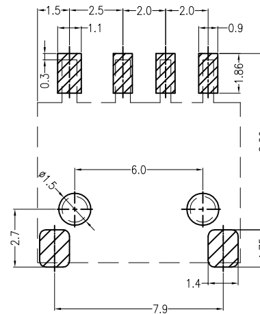
Board Layout
