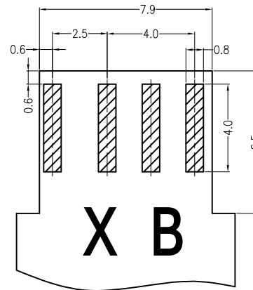
Mating Aluminum plate detail
