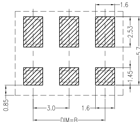
Board Layout
