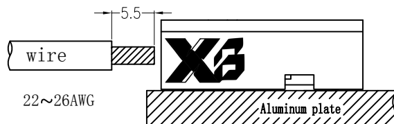
Assembly Layout
