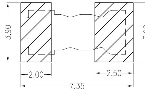
Board Layout
