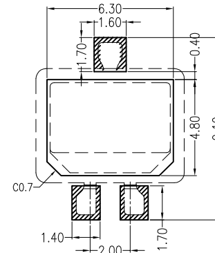
Board Layout
