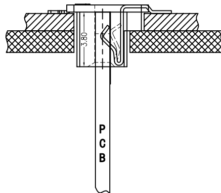
Assembly Layout
