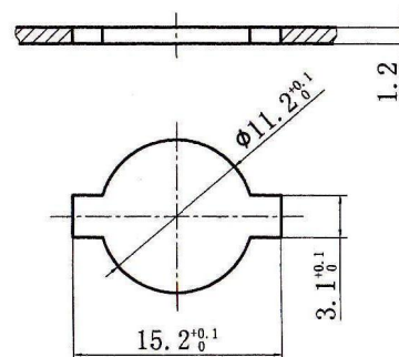
安装开孔尺寸 MOUNTING HOLE DIMENTION
