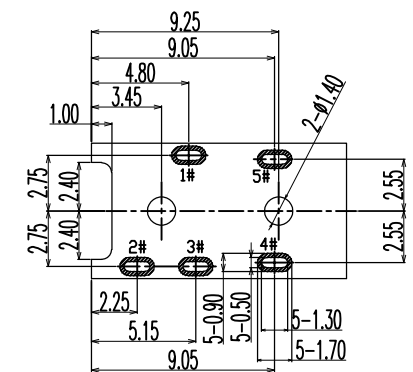
P.C.B LAYOUT T=1.00mm TOP VIEW
