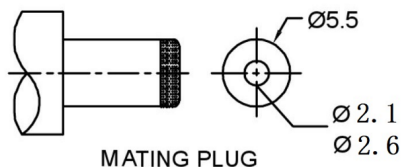
MATING PLUG
