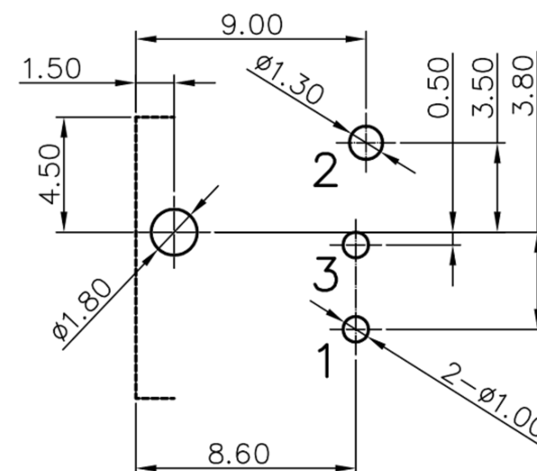
Pin Hole Layout (Jack Bottom View)
