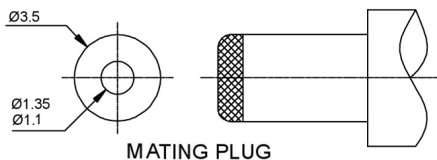
MATING PLUG
