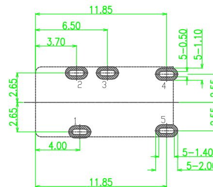
RECOMMEND FPC LAYOUT
