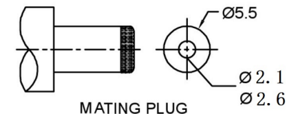
MATING PLUG
