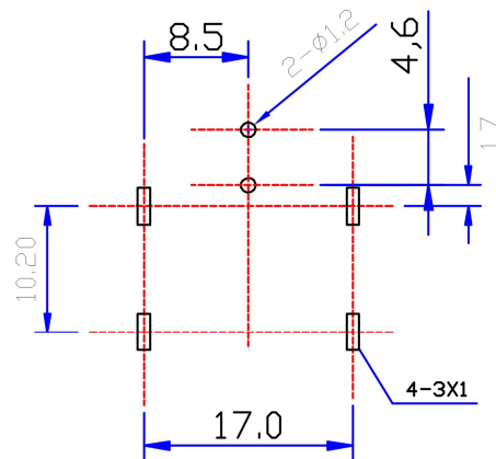
PCB LAYOUT (RECOMMENDED)
