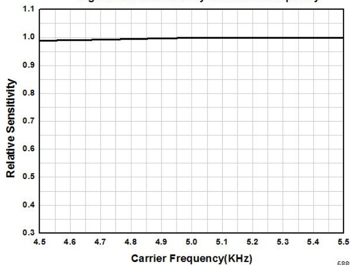
Fig.7 Relative Sensitivity vs. Carrier Frequency
