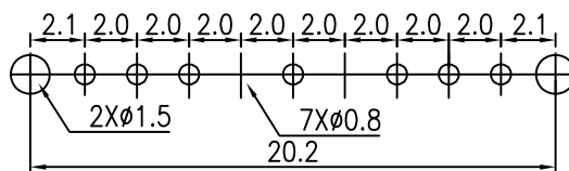
P.C.B LAYOUT TOP VIEW
