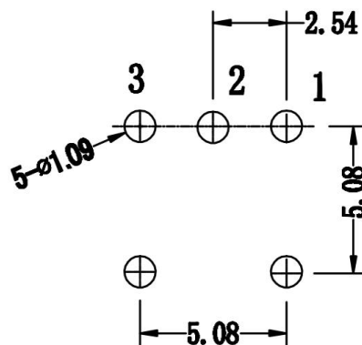
PC MOUNTING
