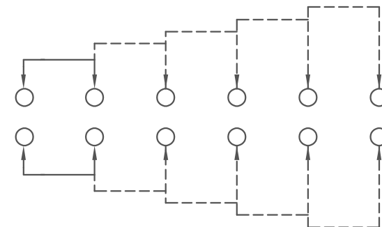
SCHEMATIC (NON-SHORTING)
