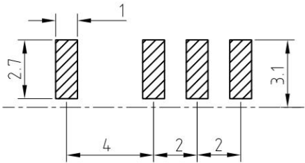
P. C. B LAYOUT
