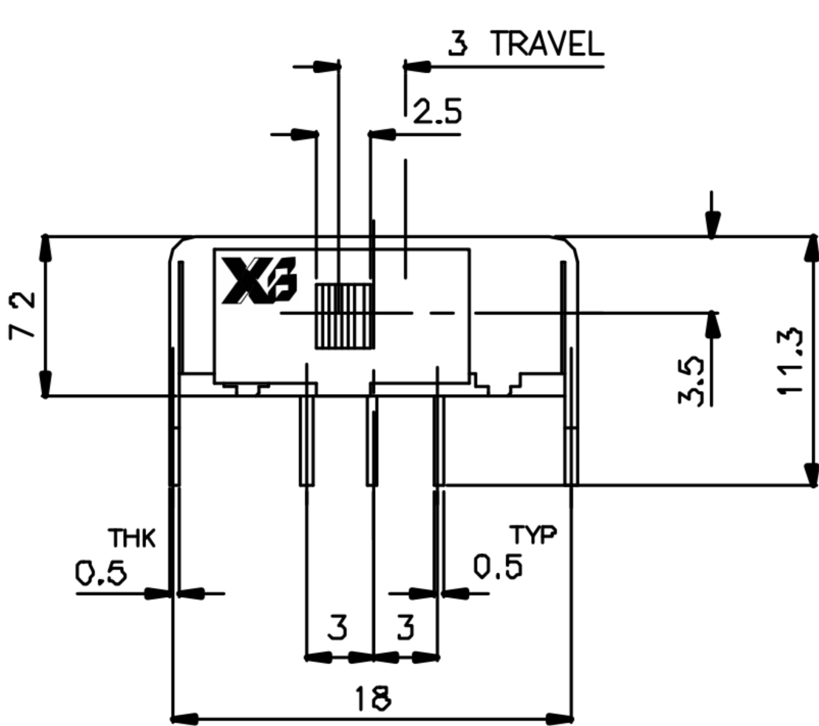
SLIDE SWITCH 1P2T
